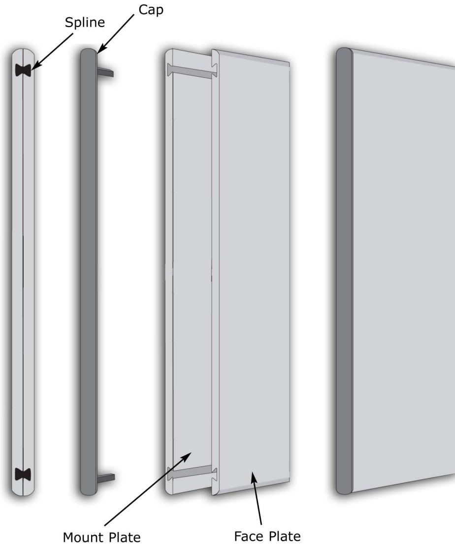
Typical End View
